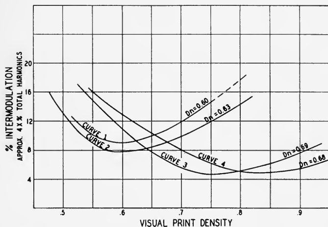
FIG. 10. Intermodulation as function of print density.
